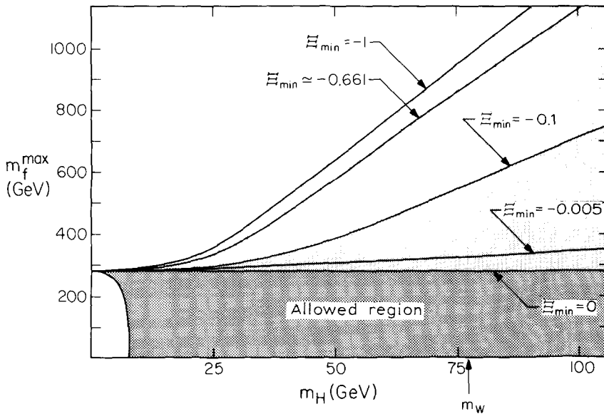
Fig. 3. The domains in the mass of the Higgs particle and of the heaviest fermion for which the Weinberg-Salam model is consistent. The value of \Xi_{\min} depends on the region of validity of perturbation theory; \Xi_{\min} is probably very small. The forbidden region in the lower left-hand corner represents the Linde-Weinberg bound.
