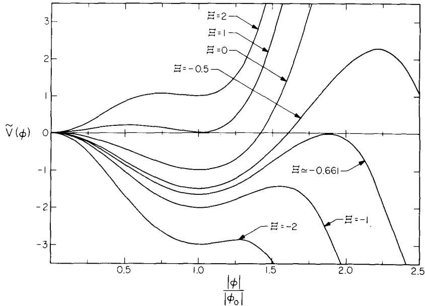
Fig. 1. The reduced effective potential \tilde{V}(\phi) = (8/m_H^2 \phi_0^2) V(\phi) as a function of \phi/\phi_0 for various choices of the combination of couplings \Xi defined in eq. (4). For usual spontaneous symmetry breakdown to occur, \phi = \phi_0 must correspond to an absolute minimum of V(\phi) , at least within the range of \phi accessible to perturbation theory.
