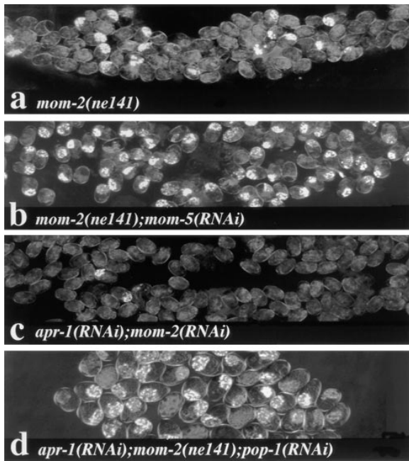
Figure 5. Endoderm Differentiation
